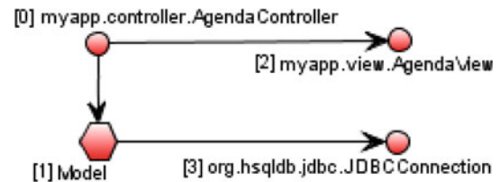
Fig. 8 myappointments' OG, with a Model domain enabled
