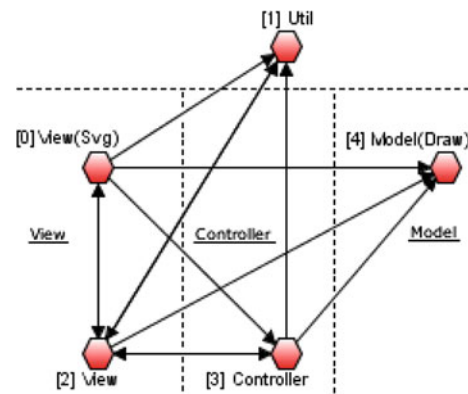
Fig. 10 JHotDraw's OG using domain-based summarization (edited to include the layer's names and dashed lines separating the layers)
