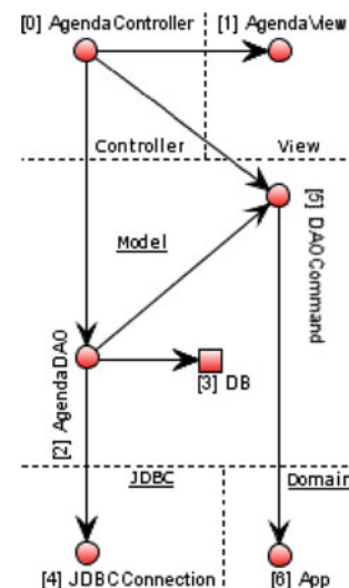
Fig. 7 Plain myAppointments' OG for the feature appointment's removal
